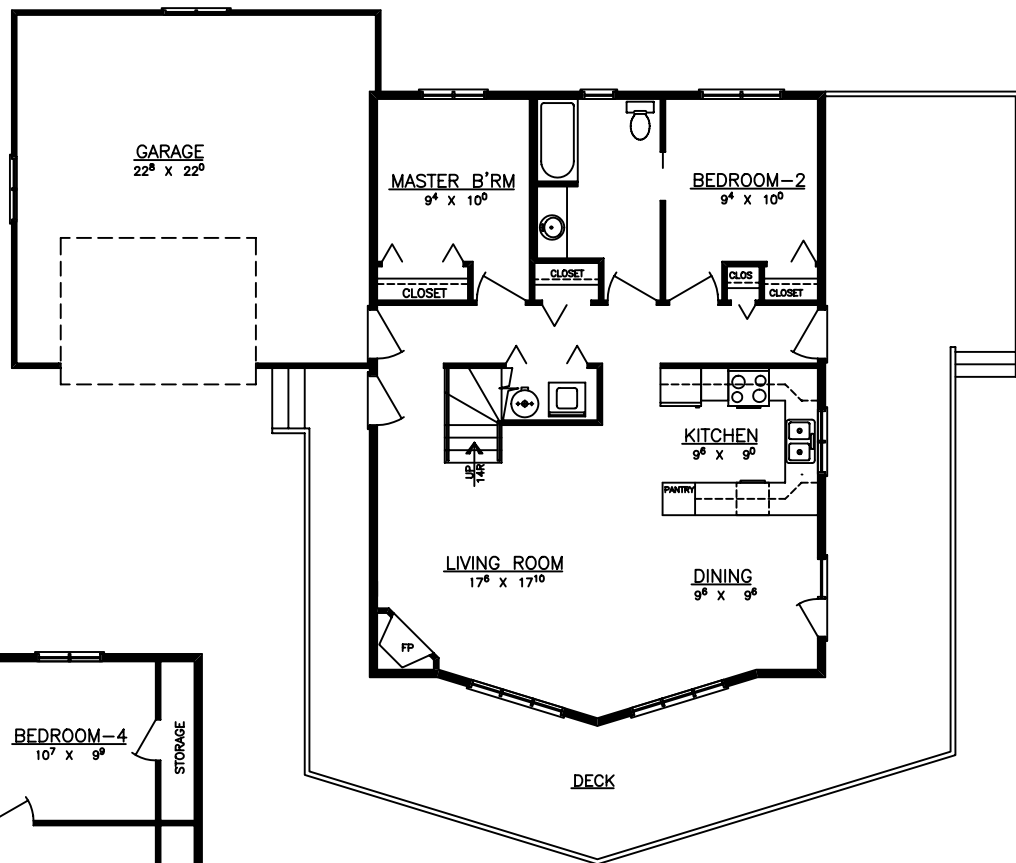
MAIN FLOOR AREA = 1038 S.F.
