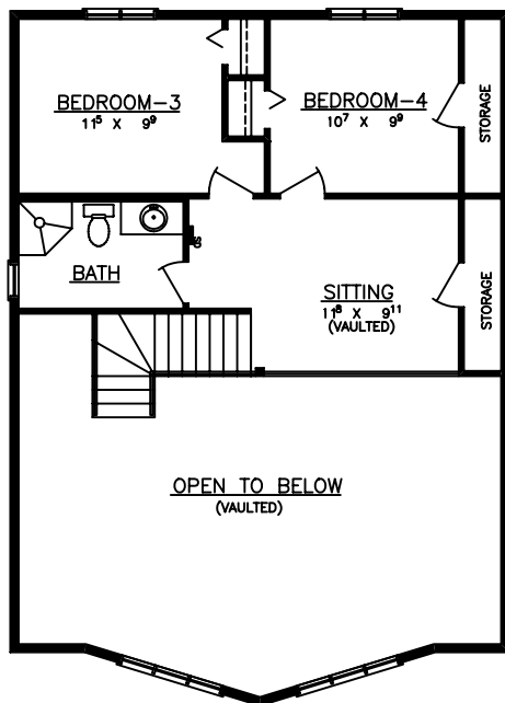
SECOND FLOOR AREA = 527 S.F.
